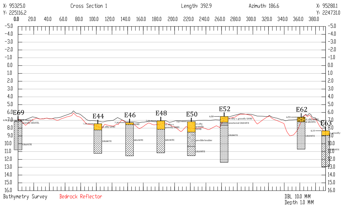
FIGURE 1: CROSS SECTIONS SCALE: VERT 1:100 HORIZ 1:1000 @ A1 (DBL VERT EXAGGERATION)
